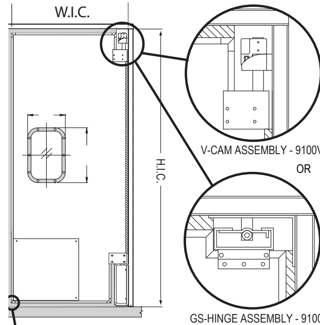
GS-HINGE ASSEMBLY - 9100
