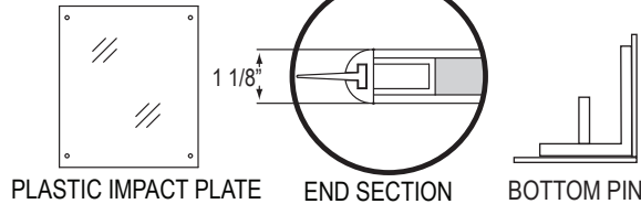
PLASTIC IMPACT PLATE
